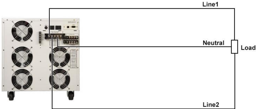
Figure 5: 1Ø3W Configuration
