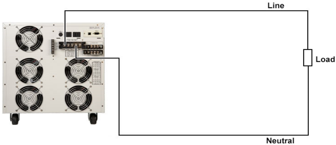
Figure 4: 1Ø2W Configuration
