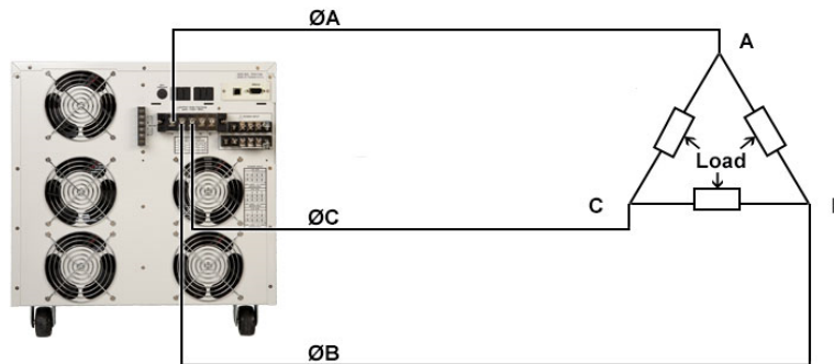
Figure 3: 3Ø3W Configuration (Delta Load)
