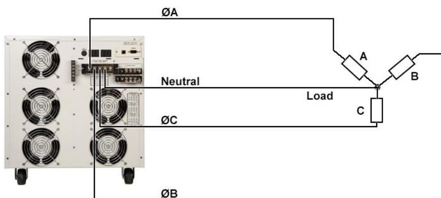
Figure 2: 3Ø4W Configuration (Wye Load)
