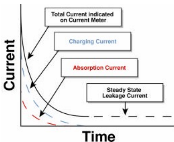
Figure 2: Direct Current vs. Time
