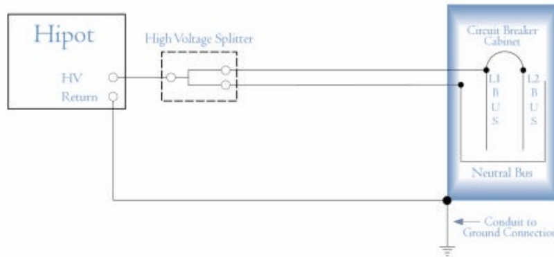
Figure 3: Hipot Tests of Manufactured and Modular Homes
